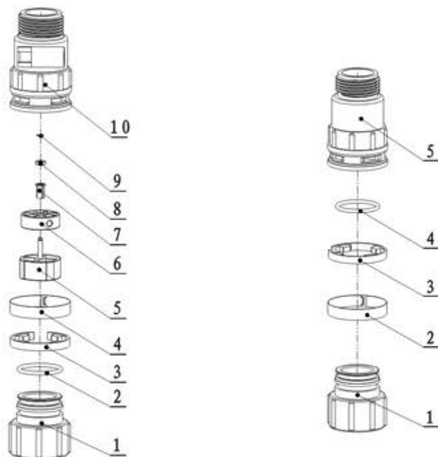
5447001 Flow Meter
